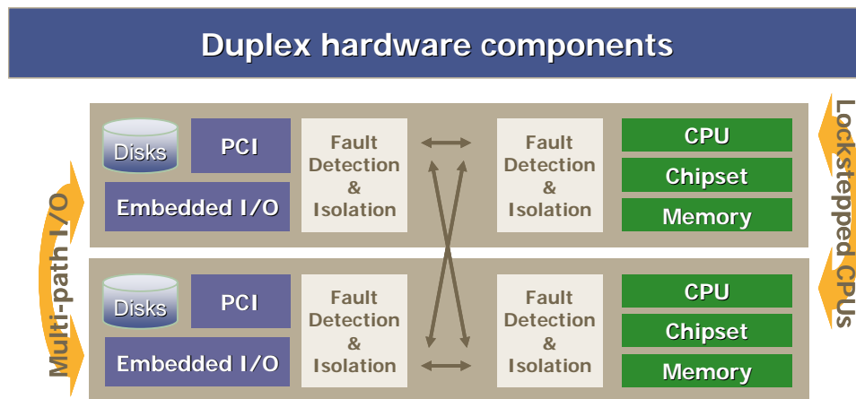
Figure 2: ftServer Lockstep Technology
